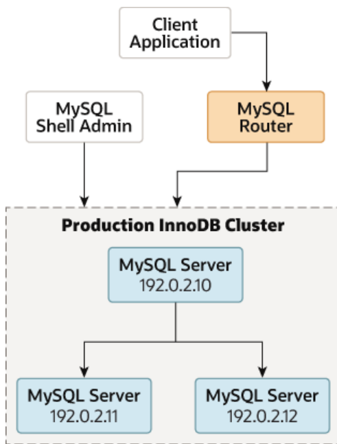
Figure 7.2 Production Deployment
