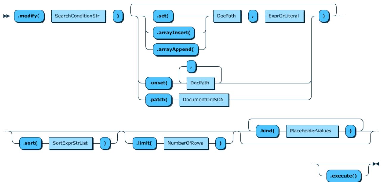
Figure 11.10 CollectionModifyFunction
